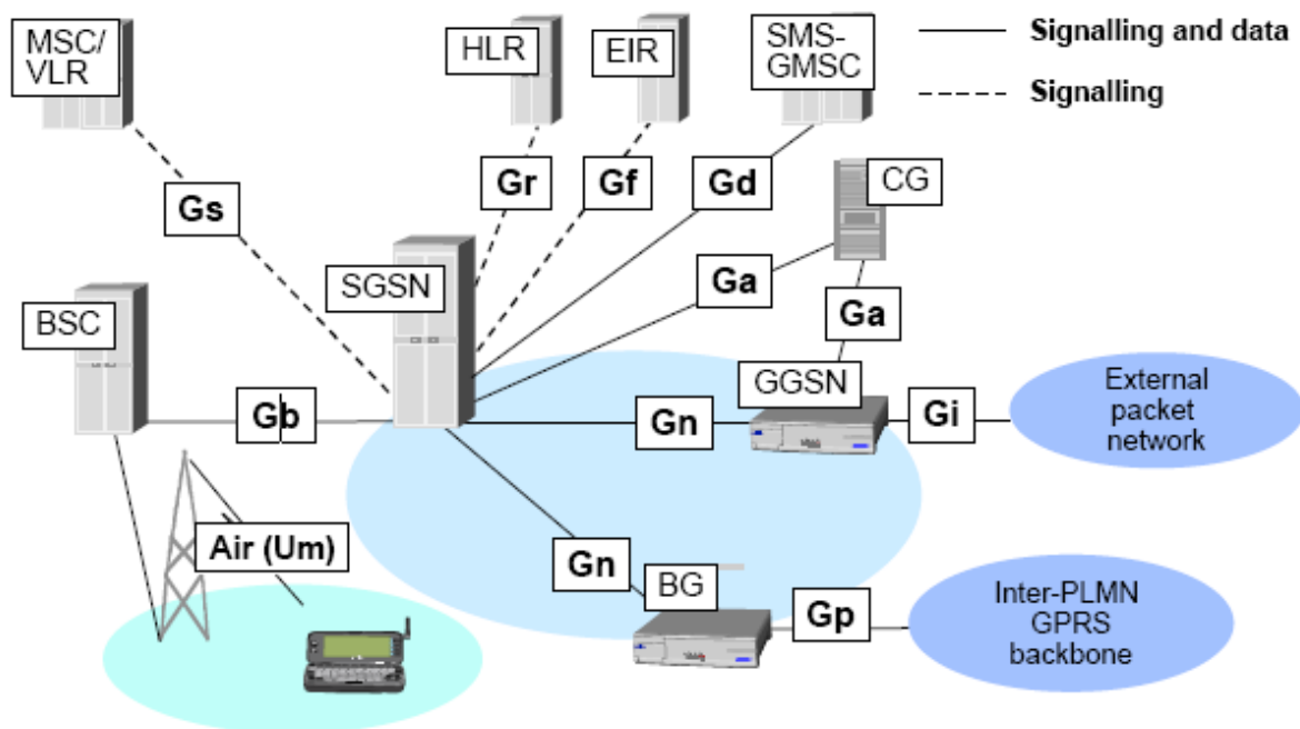
Figure 7- GPRS interfaces
