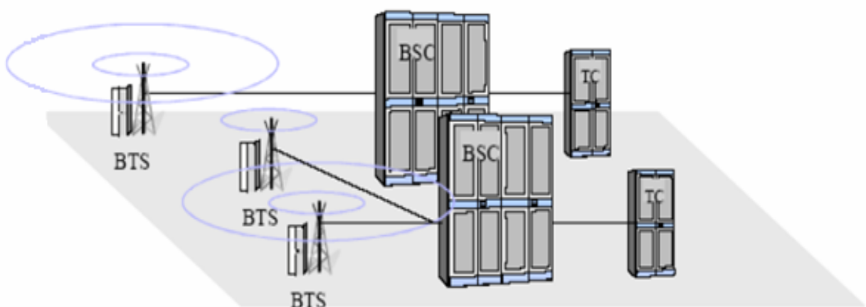
Figure 3- BSS
