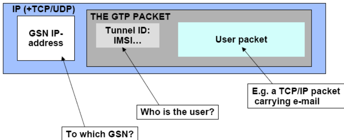
Figure 9- GTP container
