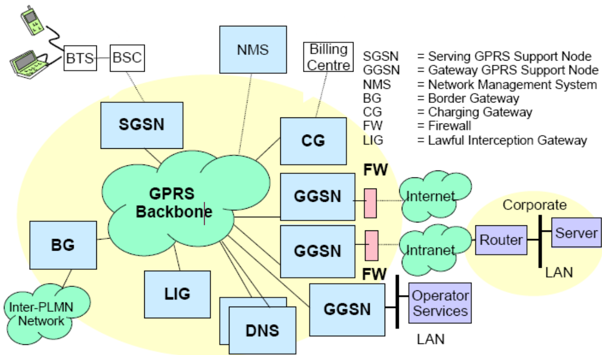
Figure 6- GPRS architecture
